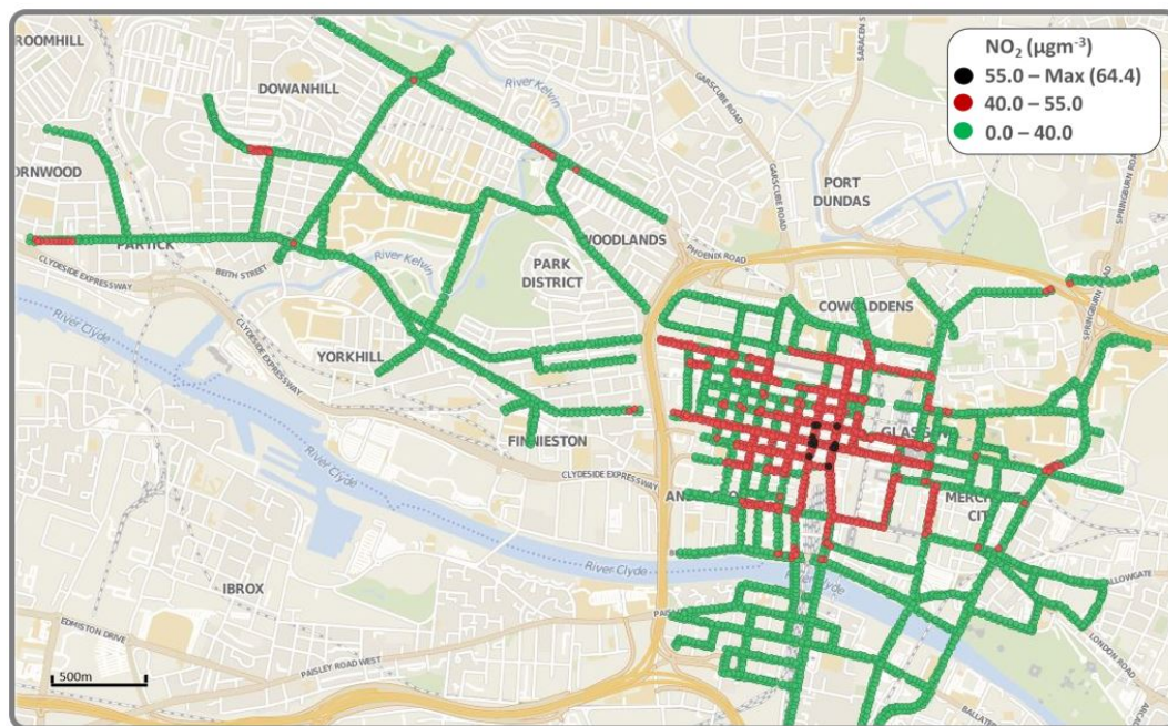
Figure 3. Modelled annual average \text{NO}_2 ( \mu\text{g m}^{-3} ) for 2019. Values greater than 40 \mu\text{g m}^{-3} (unsatisfactory) are highlighted in red and black.
