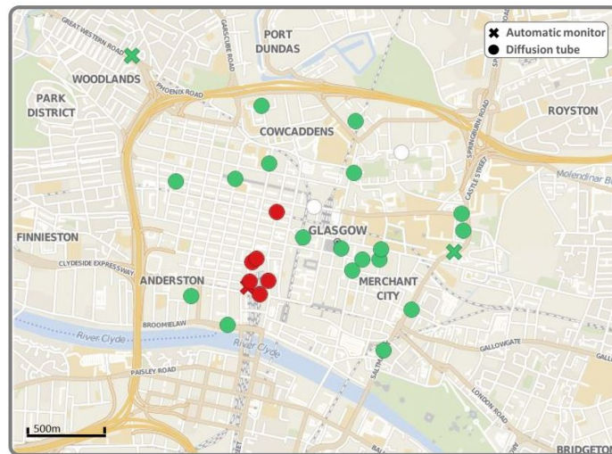
Figure 1. Annual average NO 2 concentrations at the automatic monitors and diffusion tubes within the city centre in 2018. Red markers indicate an annual average NO 2 concentration greater than 40 µgm -3 (unsatisfactory) and green markers indicate a concentration less than 40 µgm -3 (satisfactory).
